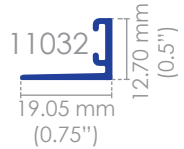
Batiente 3/4"
