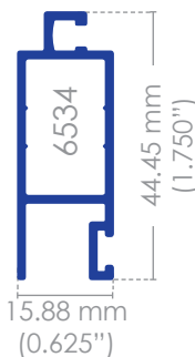
Mosquitero vertical
